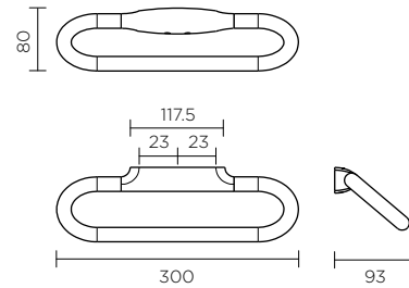
HAND TOWEL RING 428354 | Chrome › 300 x 93 x 80mm › Triple fixing points
