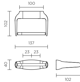
PAPER HOLDER 428352 | Chrome › 137 x 102 x 40mm › Triple fixing points
